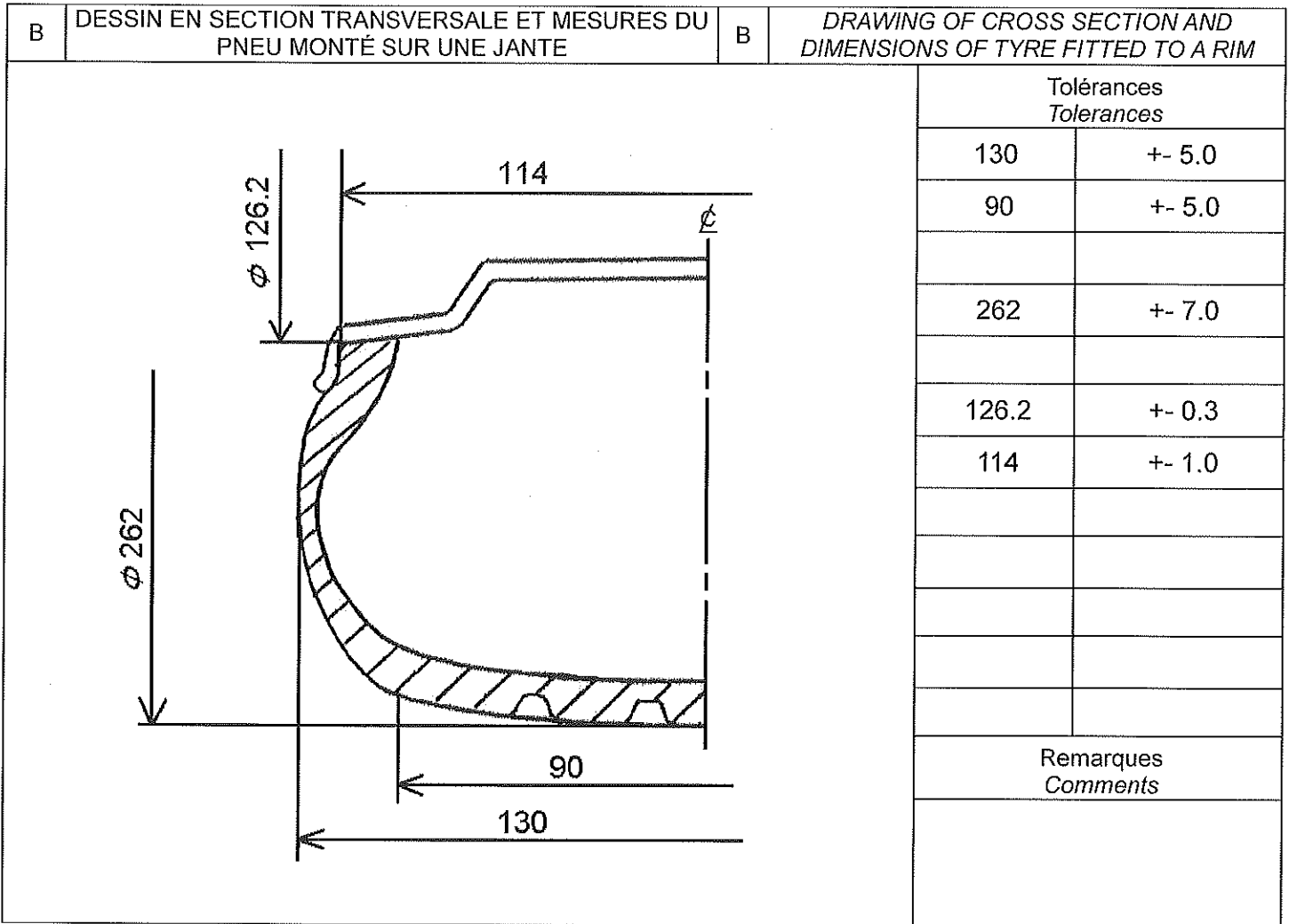
Jante 5" standardisée / Standardised 5" rim
